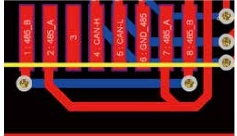
Port BMS
