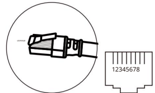
Contor-485 Port
