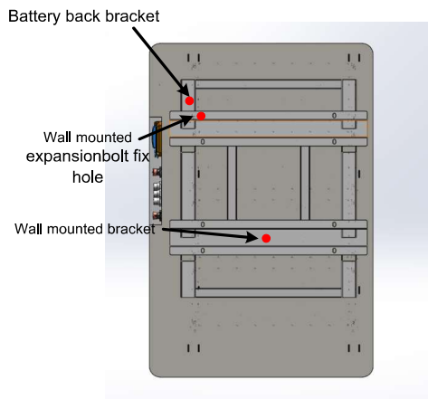
Fig. 3-1 CE48200-W PACK mechanical structure 1
