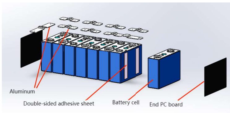
Fig. 3-2 CE48200-W PACK mechanical structure 2
