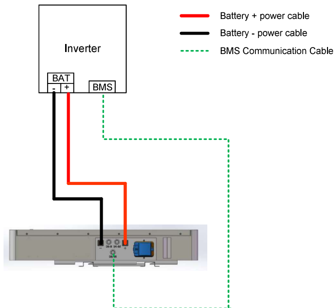
Fig. 4-1 Single CE48200-W PACK + single inverter diagram
