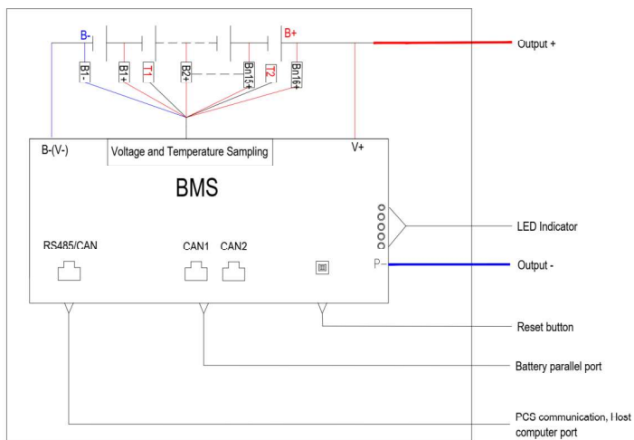
Fig. 3-4 CE48200-W PACK electrical structure
