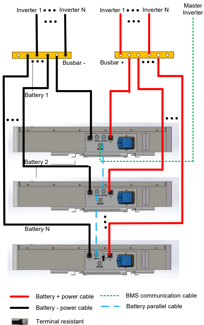
Fig. 4-2 Multi CE48200-W PACK + multi inverter diagram
