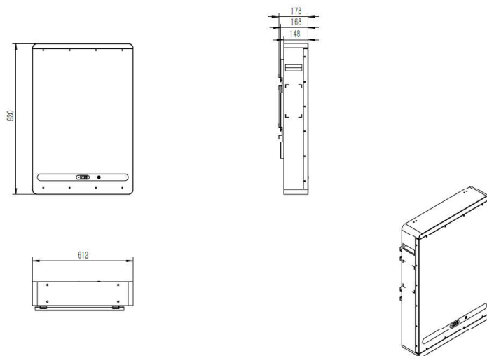
Fig. 3-3 CE48200-W PACK dimension drawing
